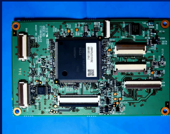
ES602G motherboard
