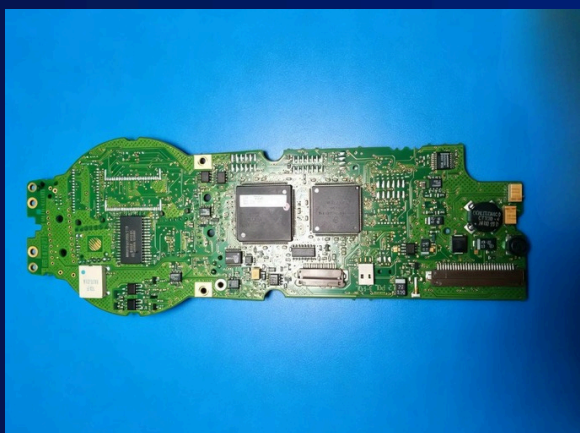
Leica total station mainboard.
