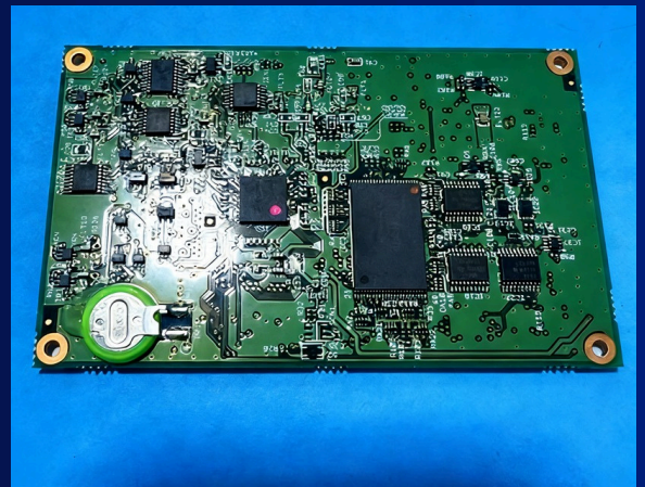
ES 600 and GTS 1000 Total Station Angle Measurement Mainboard
