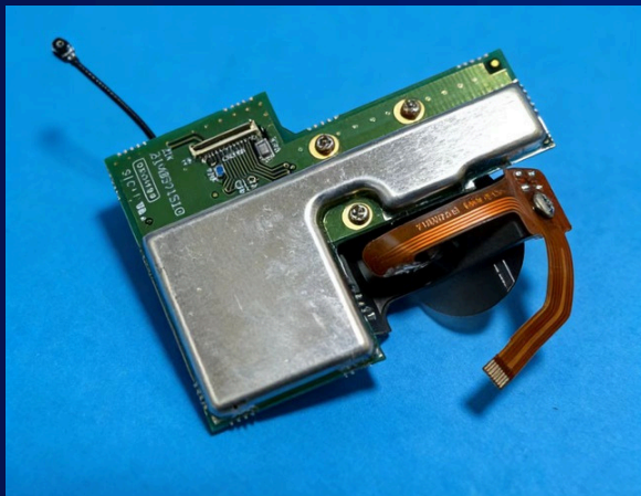
ES, GM, IM, CX, FX Distance Measurement Receiver Modules
