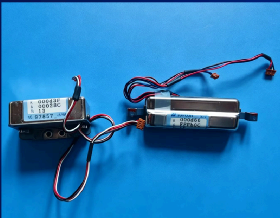
Topcon Total Station Compensator GTS330,220,250,GPT3000
